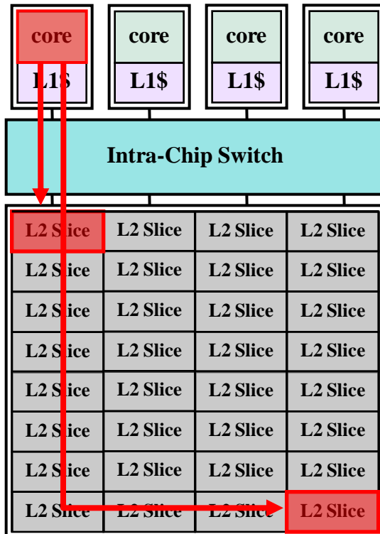
“Dance-Hall” Layout
